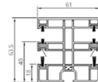
Roller guide (PVC) two-sided + MKT*. R0004
