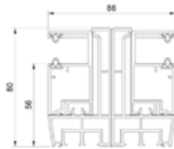
Divisive (PVC) roller guide - RS revision from the outside.
