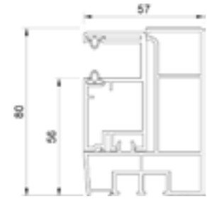
One-sided (PVC) roller guide - RS revision from the outside.
