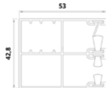
One-sided roller guide with an insect screen (for H37 and H42 laths). 87859
