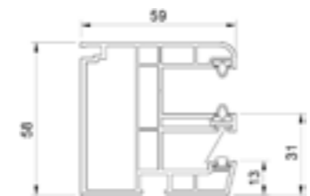
One-sided (PVC) roller guide + MKT* - RS revision from the inside.
