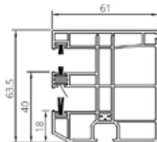
Roller guide (PVC) one-sided + MKT*. R0003
