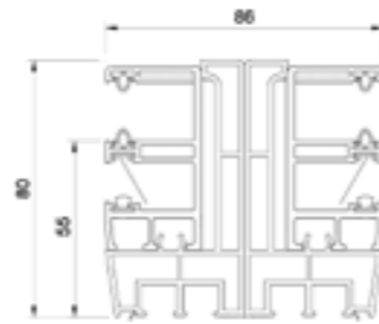
Divisive (PVC) roller guide + MKT* - RS revision from the outside.
