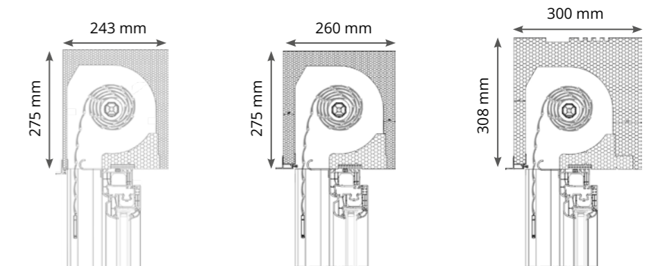
260 mm box for under the clinker.
