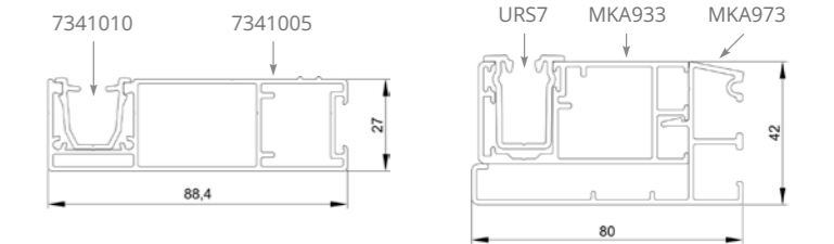
Single roller guide for ZF-A as standard.
