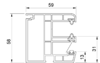
One-sided (PVC) roller guide + MKT* - RS revision from the inside. MK8110
